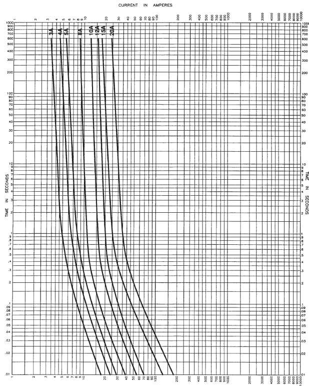
Time Curve for 3-20 Amps
