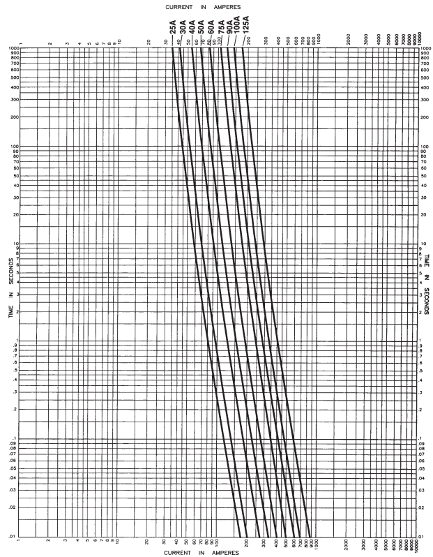
Time Curve for 25-125 Amps
